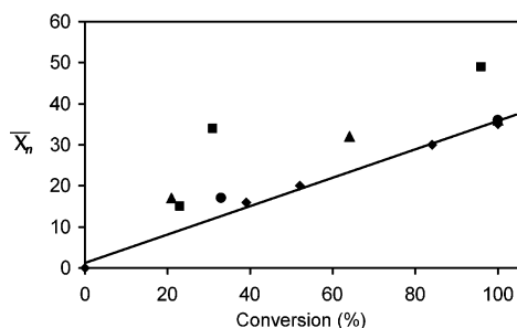
Figure 6. Evolution of the degree of polymerization with conversion for the polymerization of ethyl 1-cyanocyclopropanecarboxylate 1a using PhS − X + [X = K (◆), Na (▲), Li (■), (NBu 4 ) + (●)]; (3.8 mol % initiator; [M 0 ]/[I 0 ] = 27/1, 60 °C, \bar{X}_n obtained by GPC and corrected by NMR). The theoretical behavior expected for a living polymerization under the above experimental conditions is indicated by a solid line.
