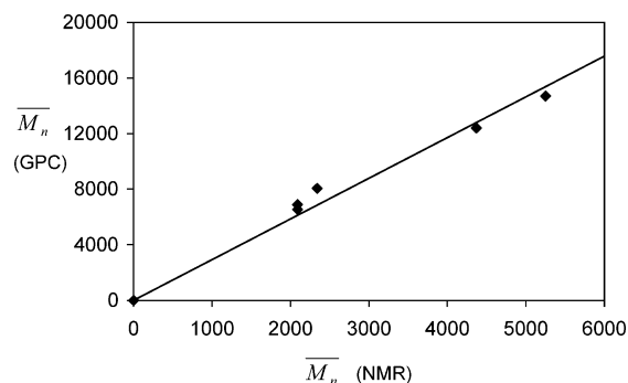
Figure 4. Comparison of \bar{M}_n values obtained from NMR and GPC for poly(ethyl 1-cyanotrimethylenecarboxylate) (poly( 1a )).
