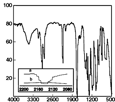
Figure 2. IR spectrum of poly(ethyl 1-cyanotrimethylenecarboxylate) (poly( 1a )); the two curves in the inset correspond to (a) the absorption arising from the propagating end-group –C(CN)(COOEt)– in a “living” polymer isolated in the regular way, i.e., the absence of any strong acid and (b) after reaction with trifluoroacetic acid.
